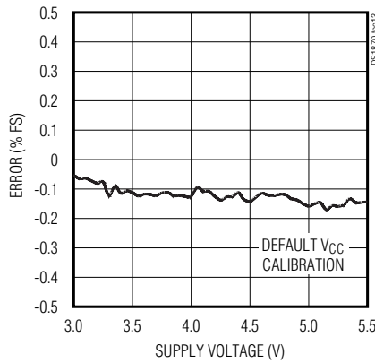
V_{CC} CONVERSION ERROR vs. SUPPLY VOLTAGE
